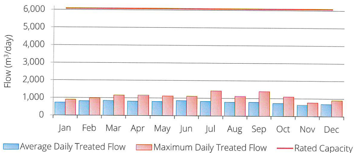
Figure 1: 2024 average and maximum daily treated water flows
